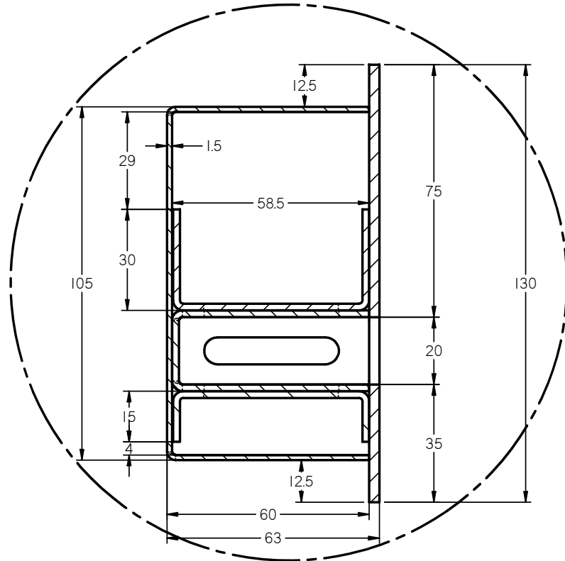
DETAIL B
